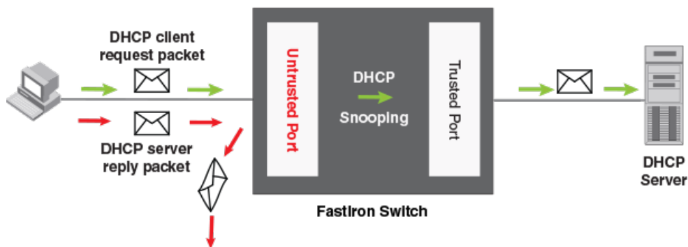
FIGURE 7 DHCP Snooping at Work on an Untrusted Port
