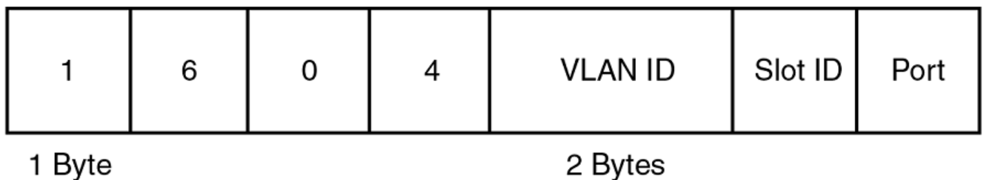
FIGURE 12 General CID Packet Format
