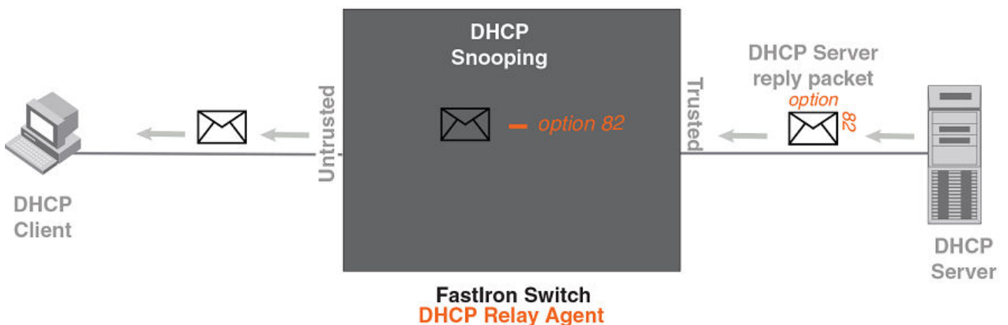
FIGURE 11 DHCP Option 82 Attributes Removed from the DHCP Packet
