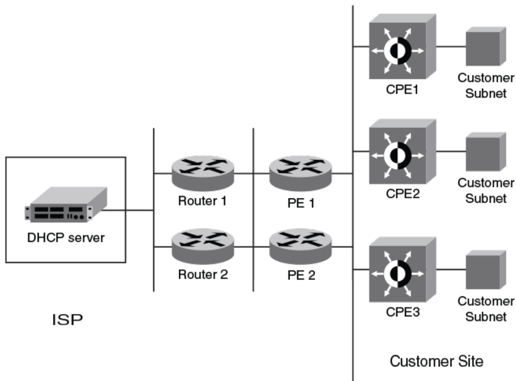
FIGURE 15 DHCPv6 Relay Agent Prefix Delegation Notification
